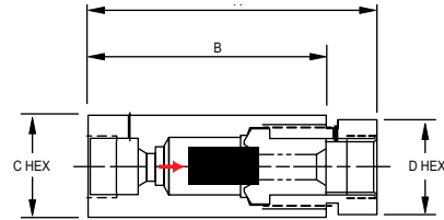
ex. 20SCF9-20
